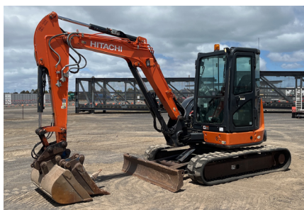
2018 Hitachi ZX48U-5A
